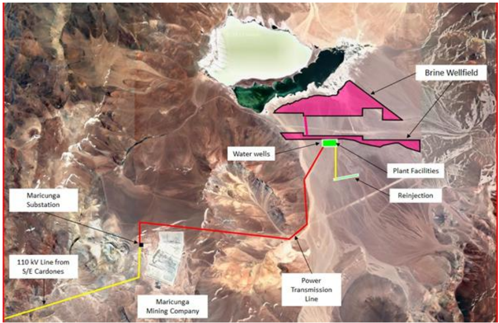
Figure 4: Scoping Study Wellfield Infrastructure Layout Plan
