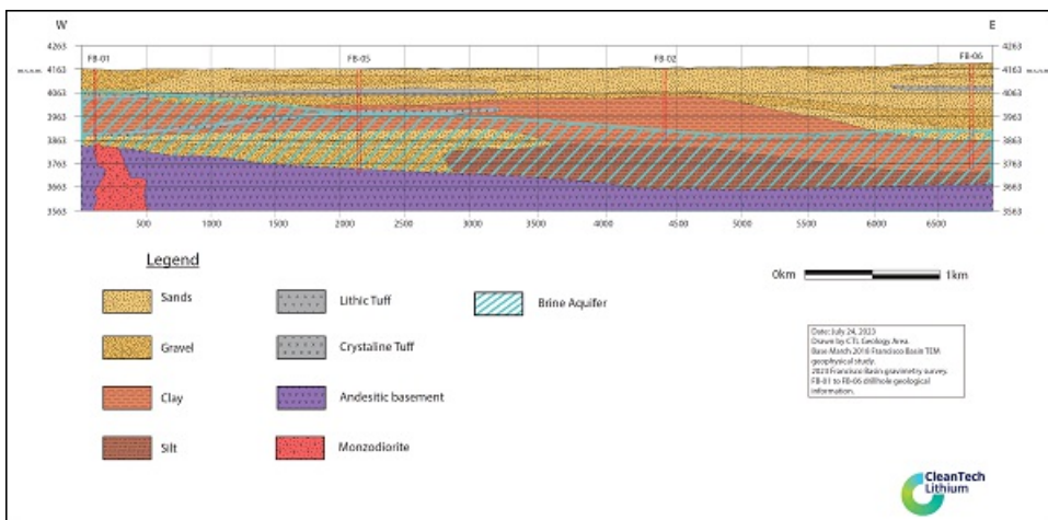
Figure 2: Francisco Basin General Stratigraphy
