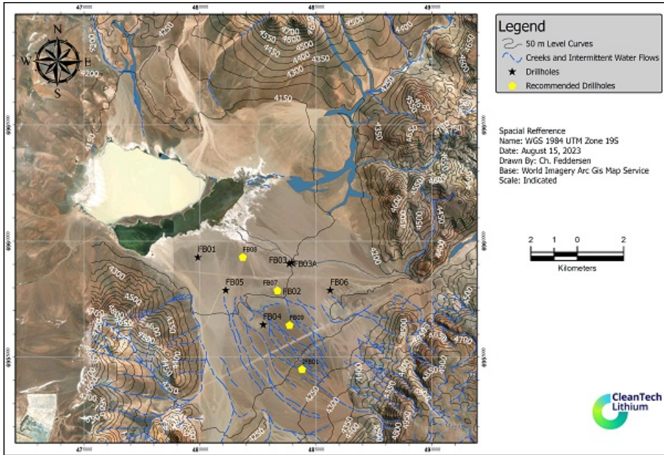
Fig 9: Francisco Basin Recommended Drillhole Locations
