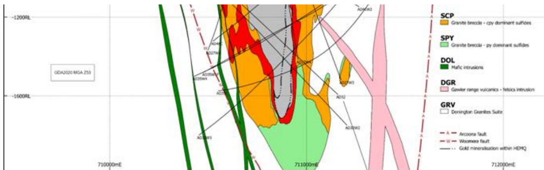
Figure 4. Representative cross-sections (6,570,980 mN)
