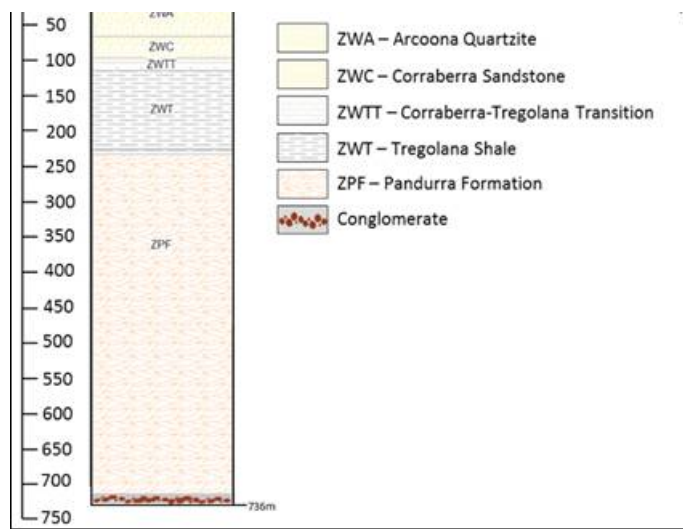
Figure 6. Simplified stratigraphic column for Oak Dam overburden.
