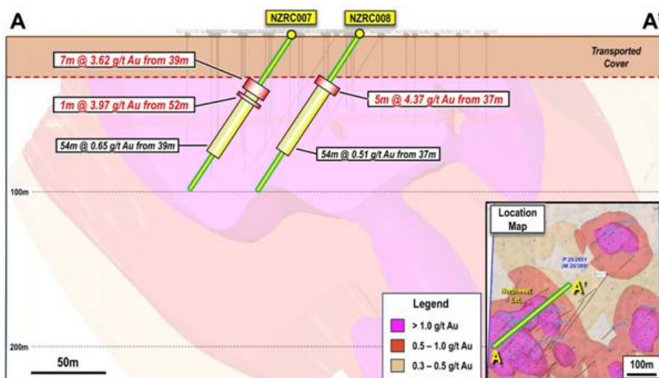
Figure 3: Cross-section of 3D Leapfrog software model The interpretation illustrates gold grade shells, derived from all the significant intercepts reported to the ASX to date. The model is constrained via a 25m buffer to all the RGL/Oracle drill hole traces that have been drilled at Northern Zone since 2021. Refer to Figure 2 drill collar plan for the location of the section line. [2]
