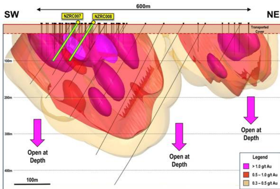
Figure 3: Cross-section of 3D Leapfrog software model The interpretation illustrates gold grade shells, derived from all the significant intercepts reported to the ASX to date. The model is constrained via a 25m buffer to all the RGL/Oracle drill hole traces that have been drilled at Northern Zone since 2021. Refer to Figure 2 drill collar plan for the location of the section line. [2]
