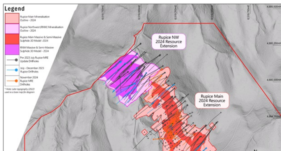
Figure 4: Plan View of 2024 Resource Block Model Outline of Rupice vs 2023 Resource Block Model
