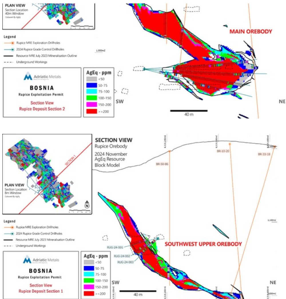
Figure 11: Cross Section #1 Rupice 2024 Resource Block Model - Southwest Upper Orebody. Extension to near surface of Rupice 'Upper' orebody.
