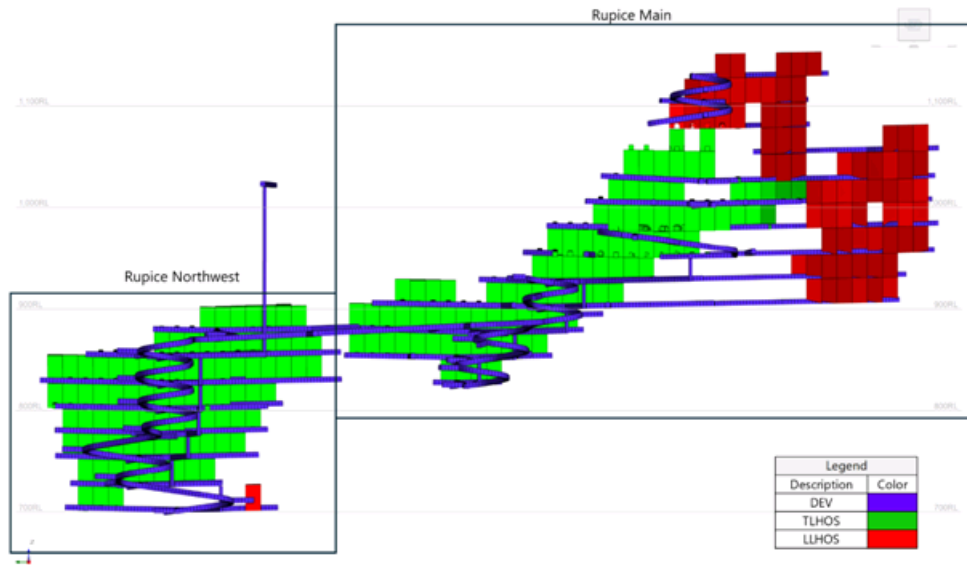
Figure 2: Mine design looking east (Adriatic Metals, 2024 Deswik Output)
