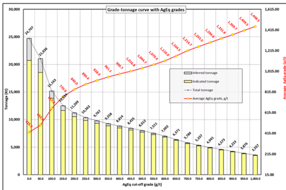
Figure 6: Grade Tonnage Curve with AgEq Grades
