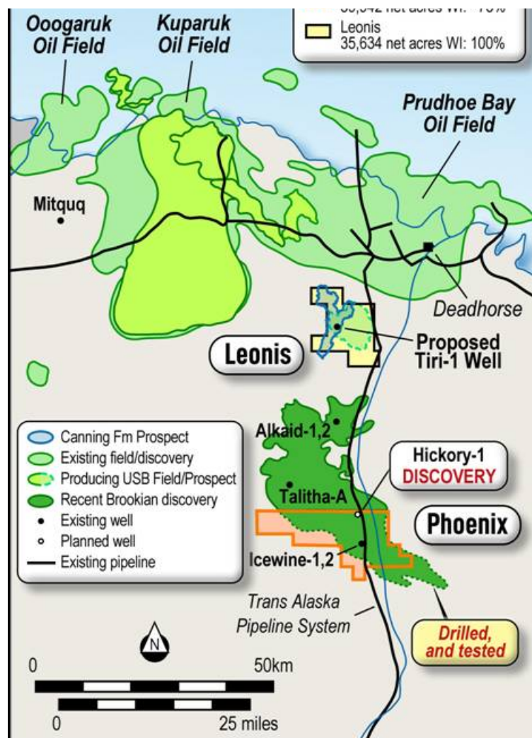
Figure 3: Alaska, North Slope, highlighting Project Phoenix and the location of the Hickory-1 discovery well.
