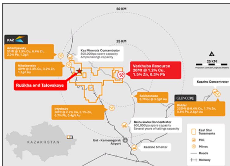
Location of East Star's projects in the Rudny Altai belt
