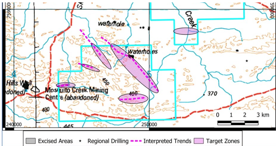
Figure 3: Highlighted Target Zones, defined by geochemical sampling and interpreted trends.
