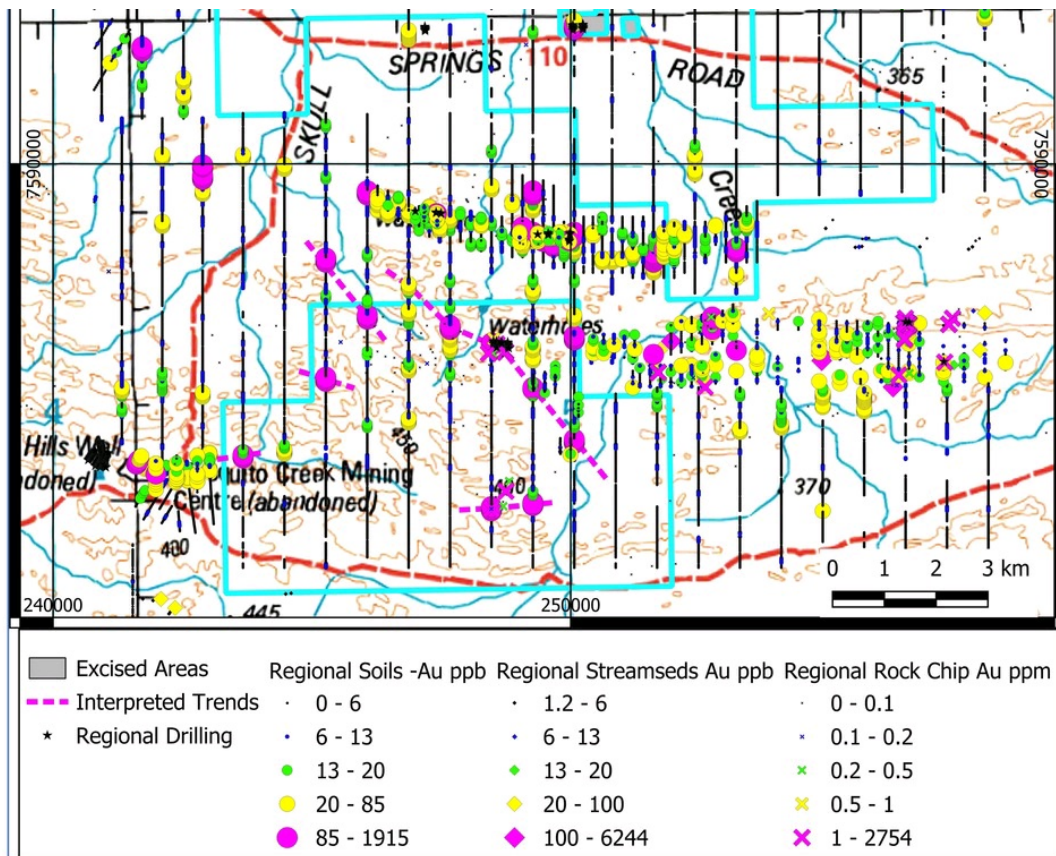
Figure 2: Compilation of all Regional geochemical sampling with interpreted trends
