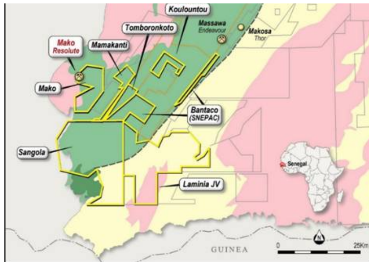
Figure 1: Senegal Geology and Project Locations
