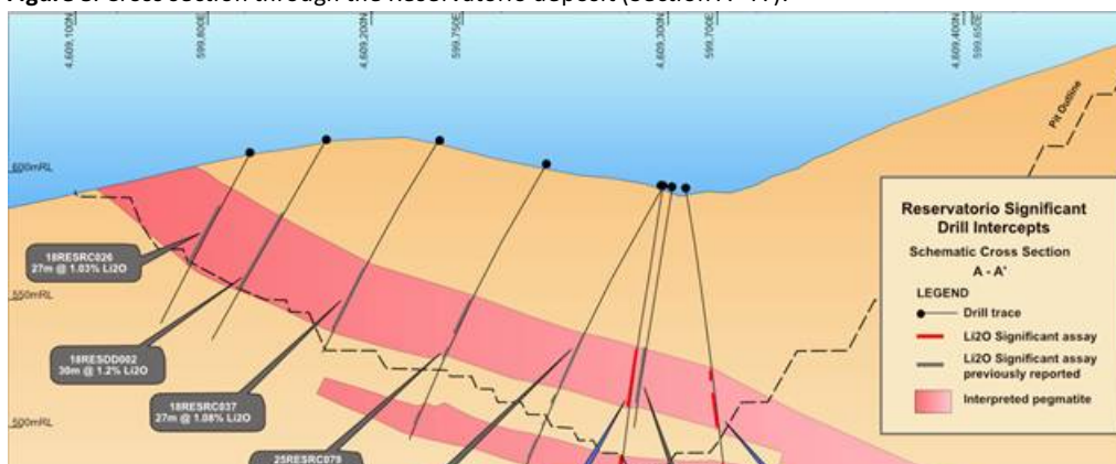
Figure 5. Cross section through the Reservatório deposit (Section A - A').
