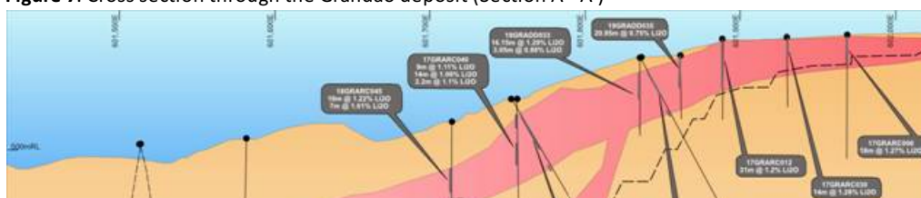
Figure 7. Cross section through the Grandão deposit (Section A - A')
