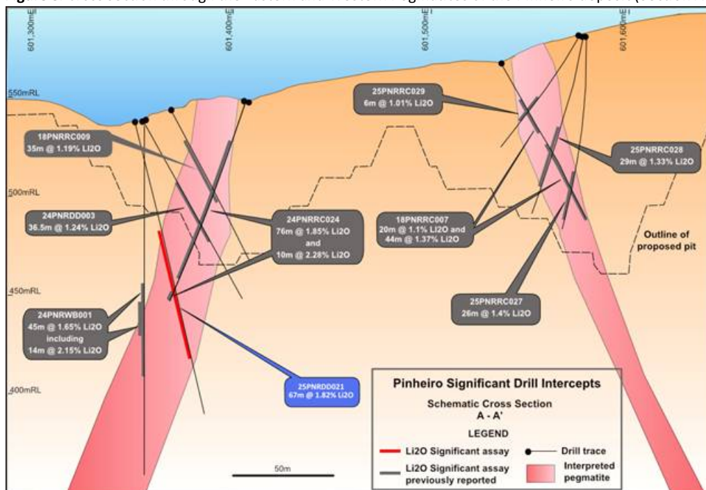
Figure 3. Cross section through the Eastern and Western Pegmatites of the Pinheiro deposit (Section A-A').
