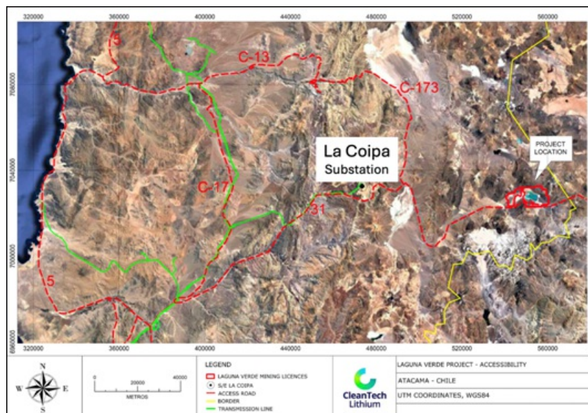
Figure 7: Route of Electrical Transmission Line based on Reference Proposal
