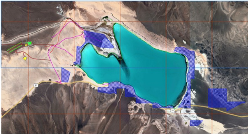
Figure 5: Area of the LiCl Plant infrastructure
