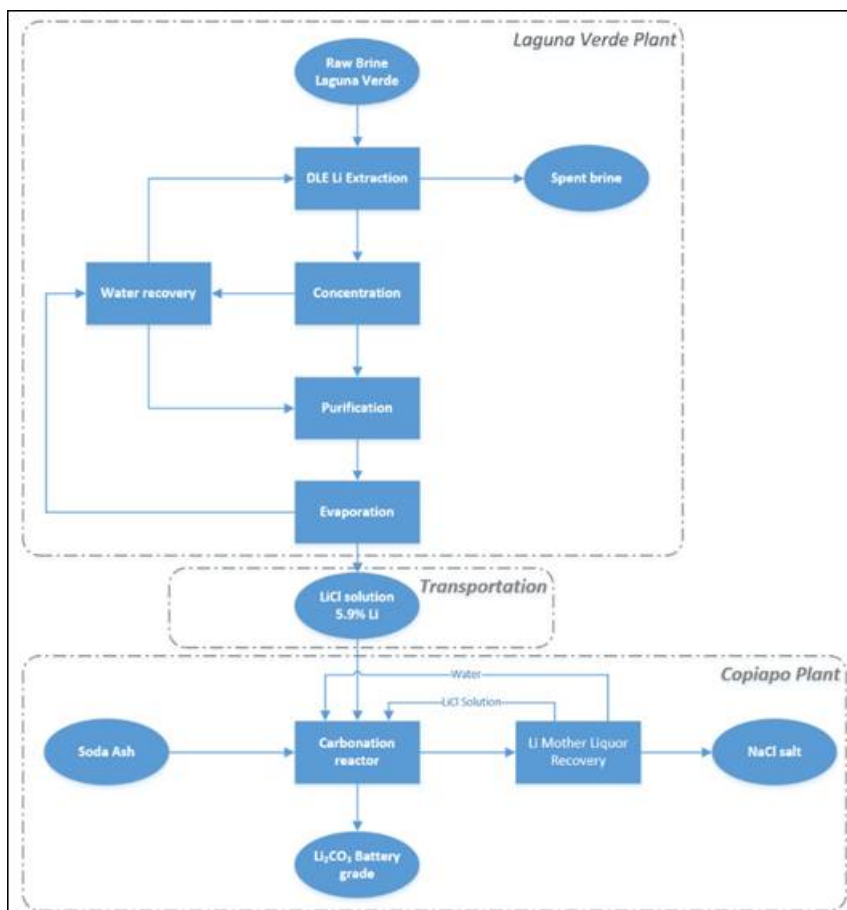
Figure 2: Process Block Diagram
