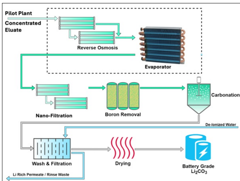
Fig. 2: Downstream process for eluate conversion
