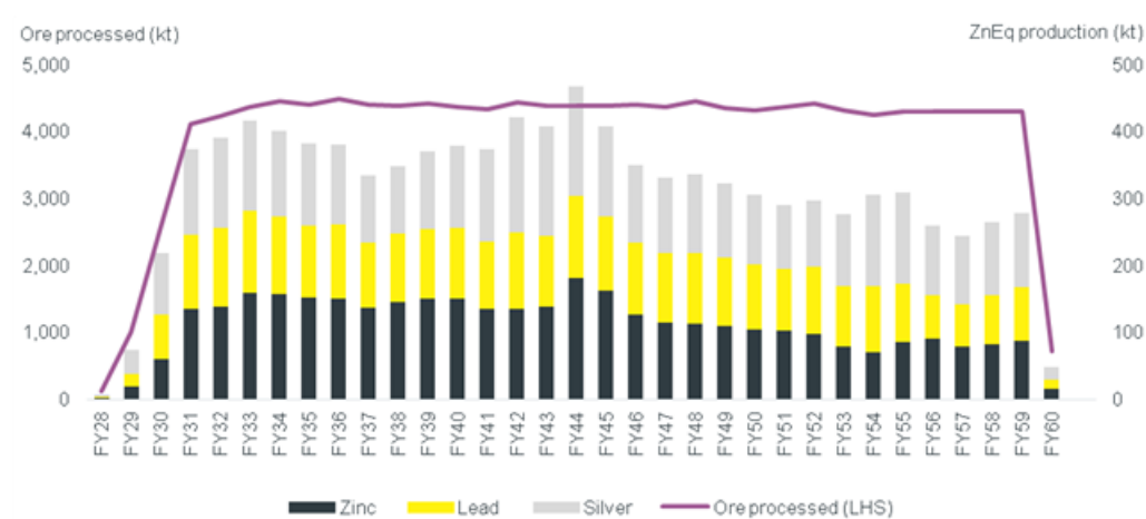
Figure 3: Ore processed and payable ZnEq production
