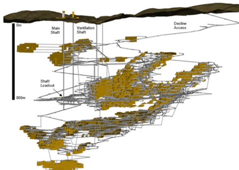
Figure 1: Taylor mine plan
