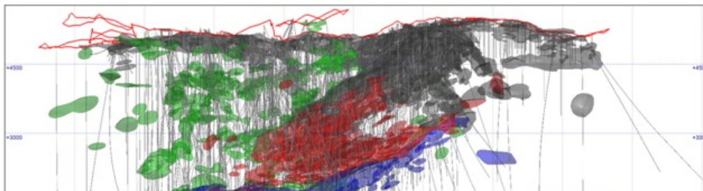
Figure 6: Oblique NE view of mineralisation domains and drilling
