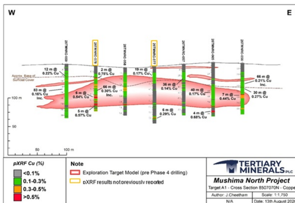
Figure 1. Cross-section (location on Figure 2) showing pXRF copper results only for new drill holes 26TMNRC-077 and 26TMNRC-078 and previously reported holes 26TMNRC-056 to 26TMNRC-059 and 26TMNRC-065, overlaid on the current Exploration Target mineralisation (silver-copper-zinc) boundary (to be updated as part of the Mineral Resource Estimation work).
