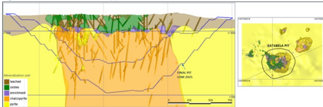
Figure 7: SW-NE Section of the Copper Mineralisation Model
