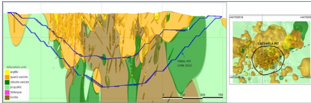
Figure 6: SW-NE Section of the Hydrothermal Alteration Model
