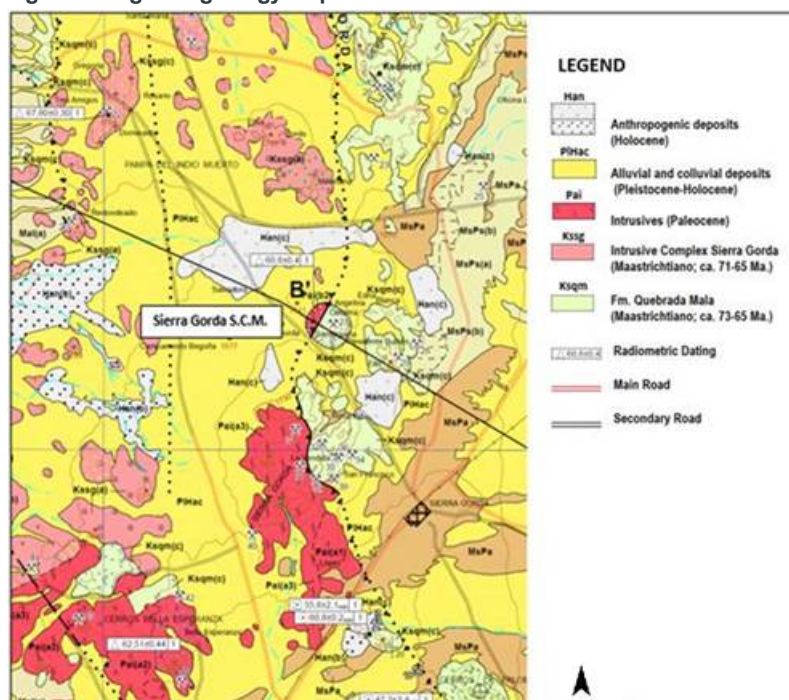
Figure 2: Regional geology map
