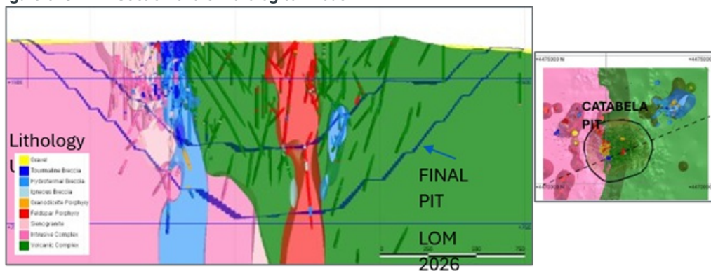
Figure 5: SW-NE Section of the Lithological Model
