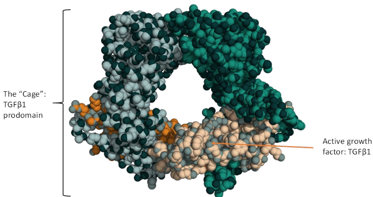
Structural representation of the latent form of TGF \beta 1 wherein the prodomain wraps around the growth factor domain
