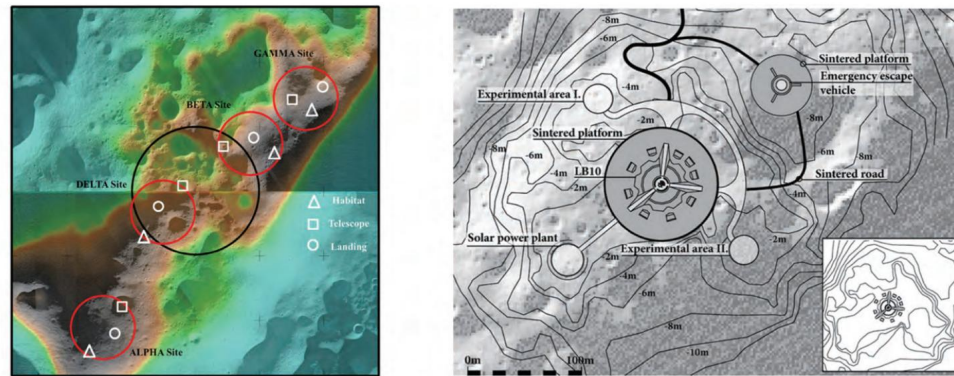
(a) 月球北极4个选址光照条件比较 (a) Illumination condition comparison of four possible sites in Moon Arctic
