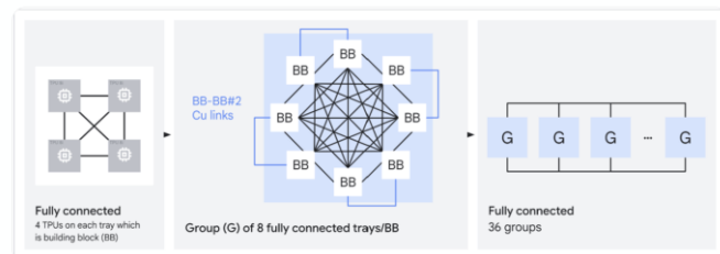
Figure 5: TPU 8i hierarchical Boardfly topology building up from a building block of four fully connected chips into a fully connected group of eight boards, with 36 of such groups fully connected into a TPU 8i pod
